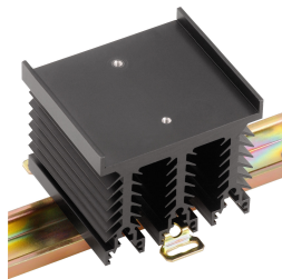
WF108110 (1.2 K/W)
